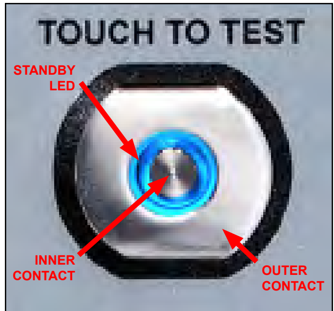
Figure 8. Steady-State Test Switch features and components
